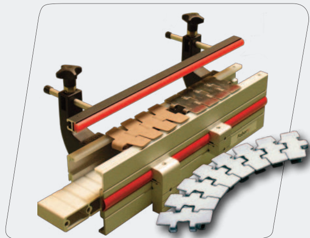
Robur with straight or curved chain
