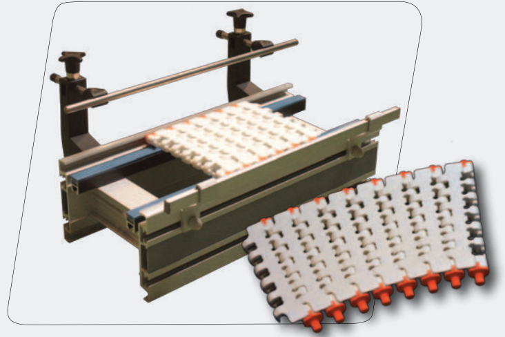
Flextoo with curved modular belt
